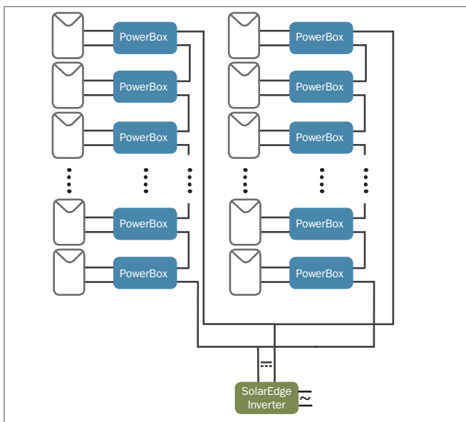
Figure 1: SolarEdge system installation
