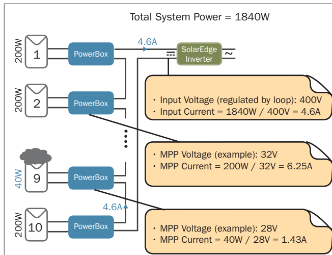
Figure 4: Operation with partial shading
