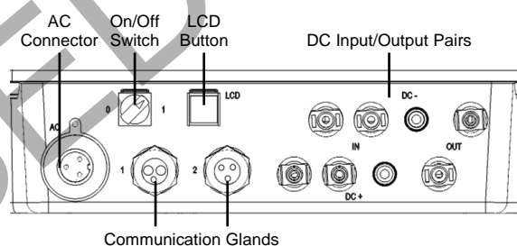
Figure 5: Safety and Monitoring Interface Connector panel
